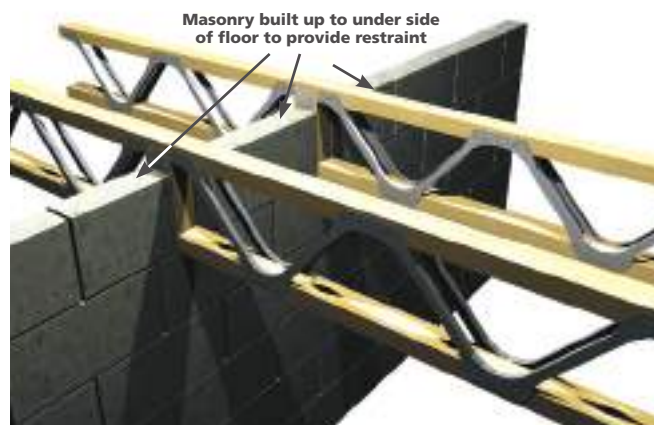
Note: This is not allowed on external walls or fire walls.
