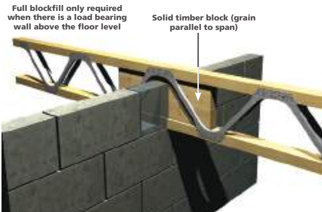
Note: This is not allowed on external walls or fire walls.
