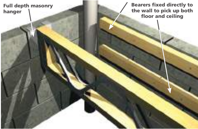
Top chord restraint omitted for clarity.
