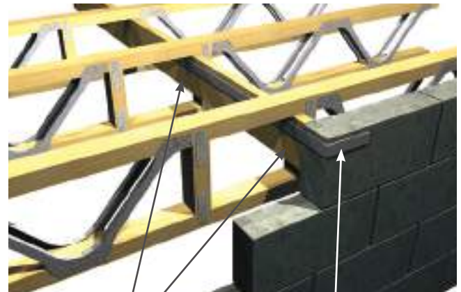
Strongback twice nailed to brace using 3.1x75mm long galvanised wire nails
